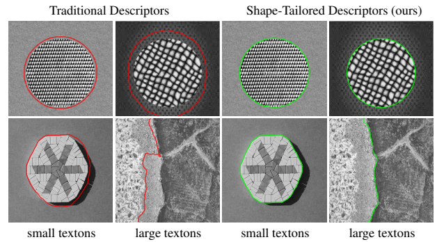
Figure 1. [Left]: Descriptors that aggregate local image data across boundaries of textured regions lead to segmentation errors. The problem is exacerbated as the texton size increases. [Right]: Segmentation by Shape-Tailored Descriptors (our method).
