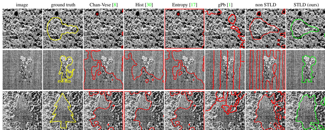
Figure 4. Sample Results on the Synthetic (Brodatz) Texture Dataset.
