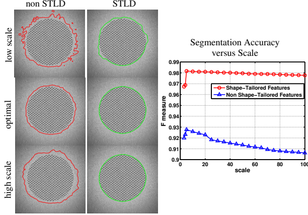
Figure 3. Robustness of Shape-Tailored Features to the Choice of Scale. [Left]: a synthetic image is segmented using low, optimum and large scales for non-STLD and STLD. [Right]: the accuracy of segmentation as the scale of the descriptor is increased. Larger F-measure indicates a more accurate segmentation.
