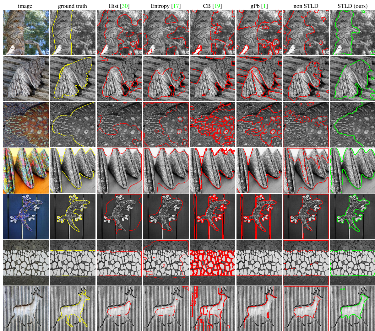
Figure 5. Sample Results on the Real Texture Dataset. Segmentation boundaries are displayed for various methods.
