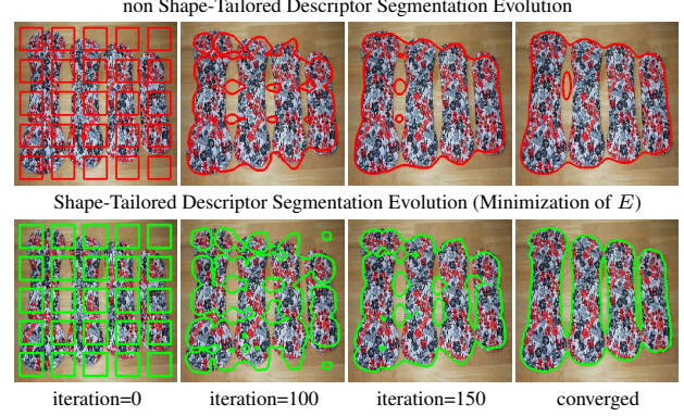
Figure 2. [Top]: non shape-tailored (traditional) local descriptors segmented with Chan-Vese. [Bottom]: segmentation of Shape-Tailored Descriptors with the piecewise constant model.
